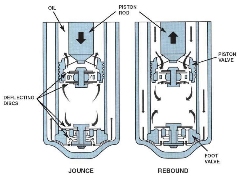
FIGURE 5-49 Oil flow through a deflected disc-type piston valve. The deflecting disc can react rapidly to suspension movement. For example, if a large bump is hit at high speed, the disc can deflect completely and allow the suspension to reach its maximum jounce distance while maintaining a controlled rate of movement.
