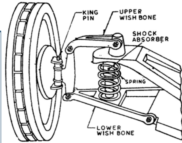
Wishbone type independent suspension.
