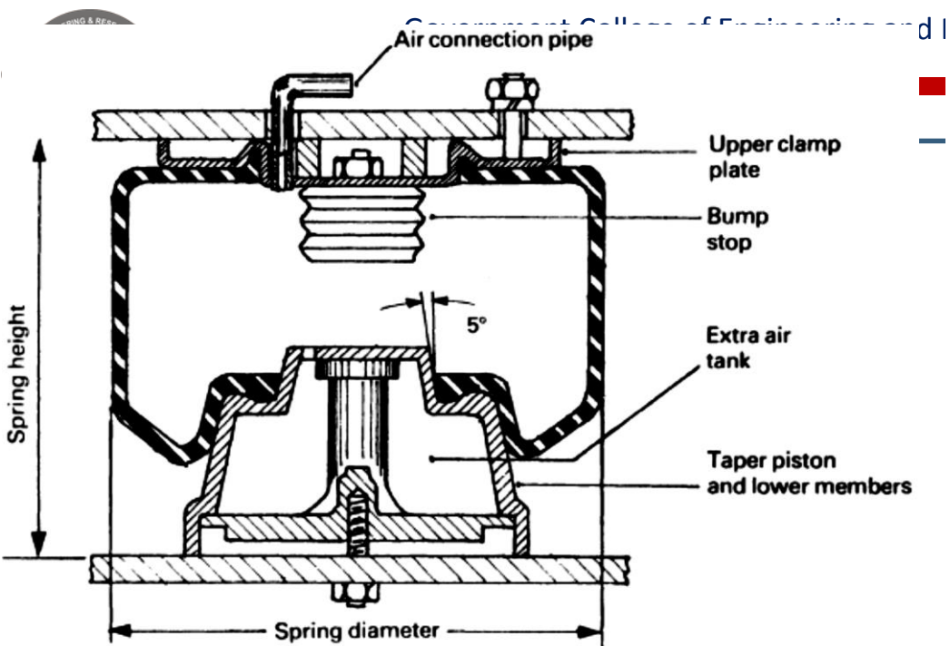
Rolling Lobe/Diaphragm
