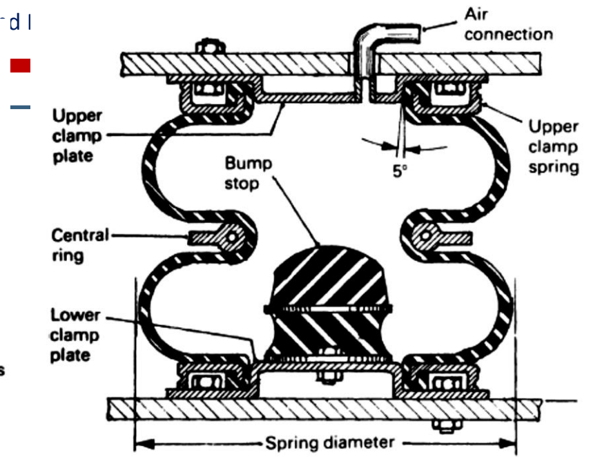
Involute/Double Convolute Spring
