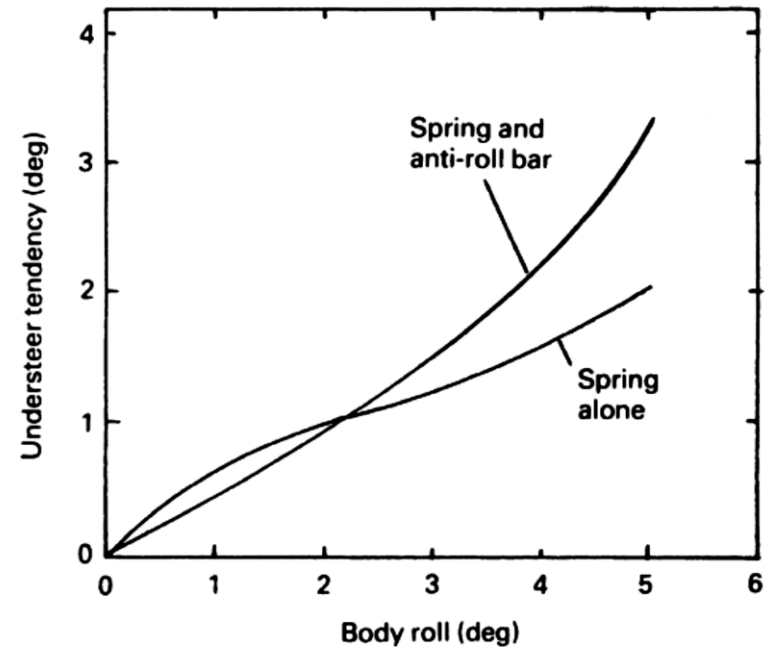
Fig. 10.38 Relationship of body roll and the understeer tendency with and without an anti-roll bar
