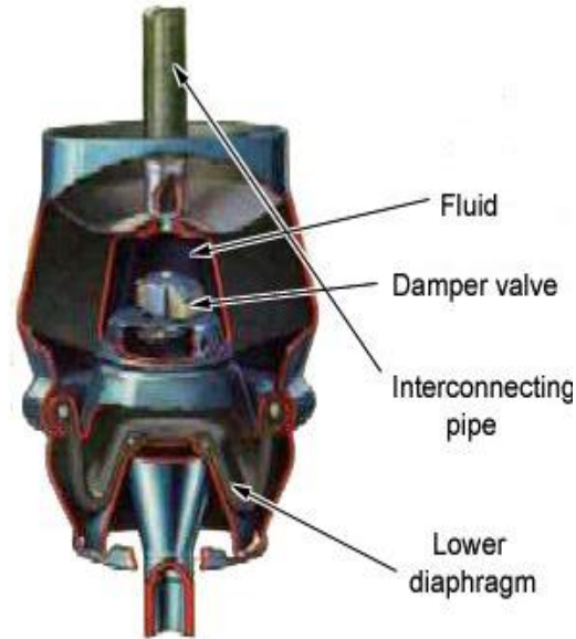
Hydrolastic displacer
